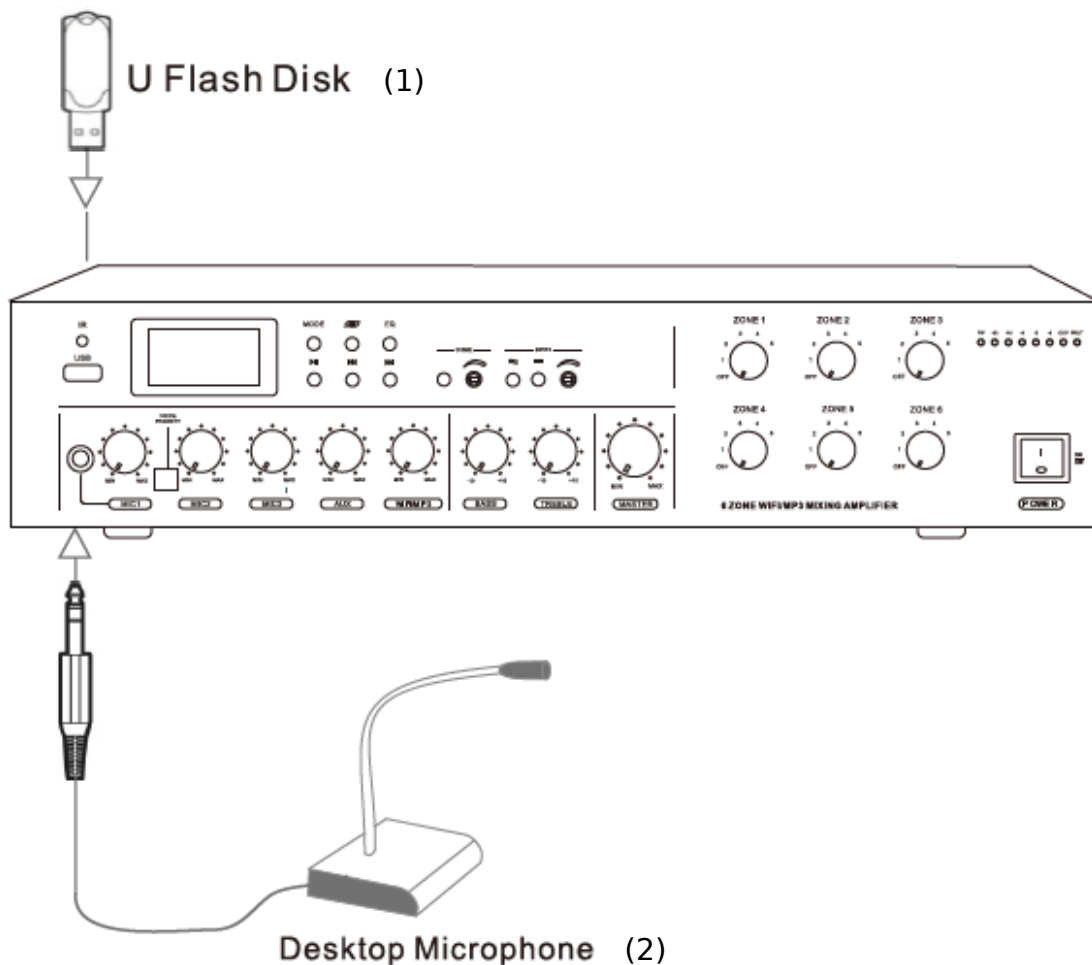
Front Panel
